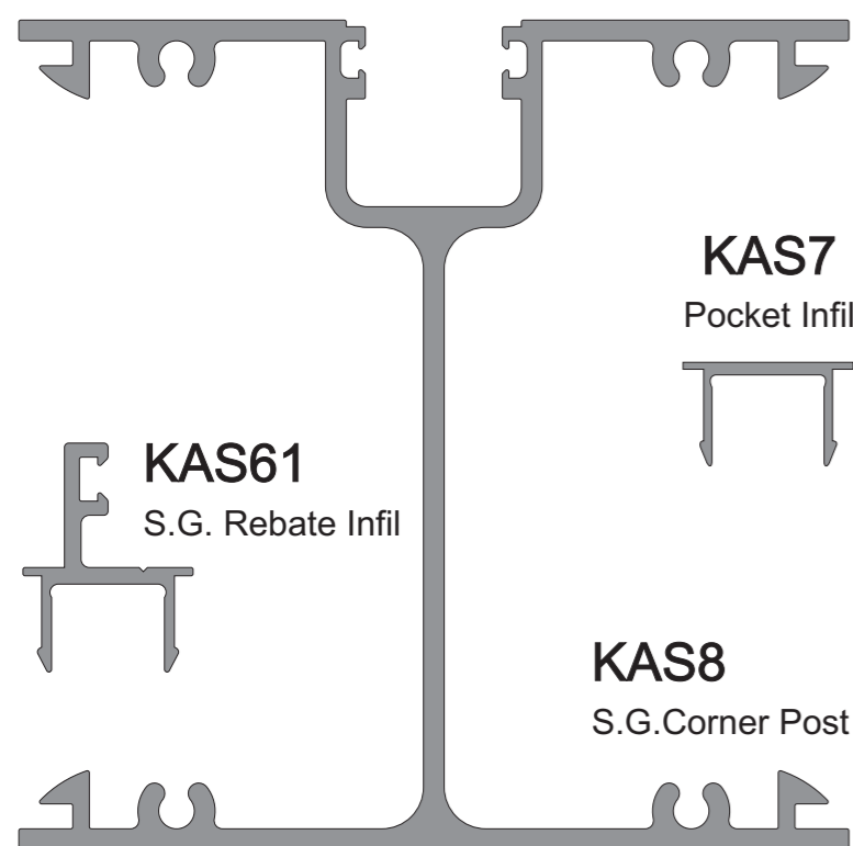
KAS70 S.G. Shallow Frame
