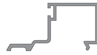
KAS56 Rebate Bead
