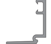
KAS32 28mm Bead
