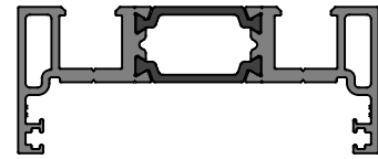
KAS743 Adjustable Outer Jamb
