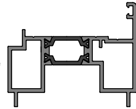
KAS7405 Double Door Add On Profile
