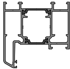
KAS732 Stile / Frame
