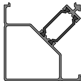
KAS614 70mm Corner Post
