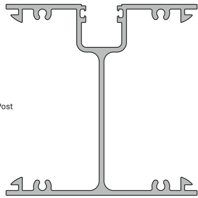
KAS46 Double Glaze Corner Post
