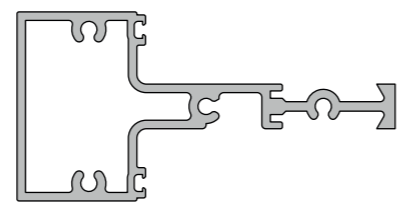
KAS48 Double Glazed Transom
