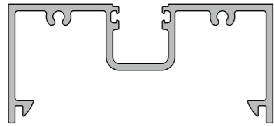
KAS1 Single Glaze Pocket Frame
