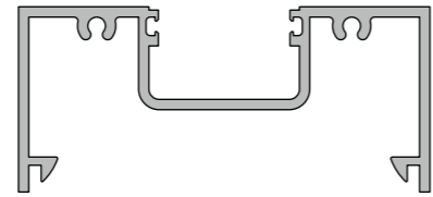
KAS41 Double Glaze Pocket Frame
