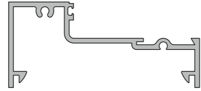
KAS42 Double Glaze Cill
