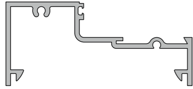
KAS3 Single Glaze Cill
