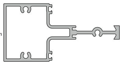
KAS78 Single Glaze Transom
