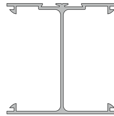
KAS54 Corner Post
