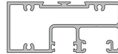
KAS65 Folding Door Header Track
