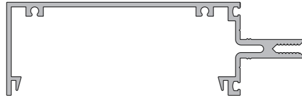
KAS821 125mm Mullion
