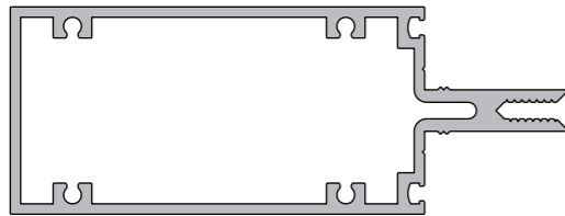
KAS814 100mm Box Transom
