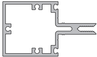
KAS805 50mm Box Transom
