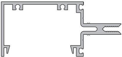
KAS801 75mm Mullion
