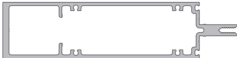
KAS826 175mm Box Transom
