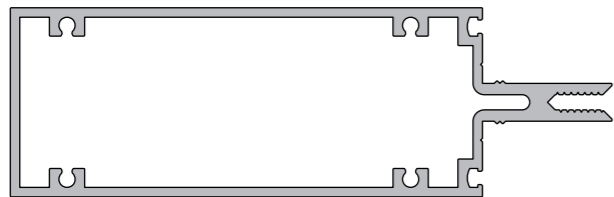
KAS824 125mm Box Transom
