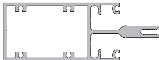
KAS831 100mm Roof Bar
