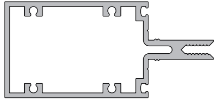
KAS804 75mm Box Transom
