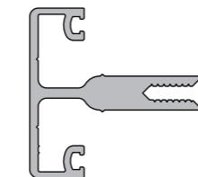
KAS832 Roof Purlin
