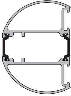
KAS763 Bottom Rail
