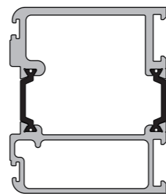
KAS765 Concealed Vertical Rod Stile
