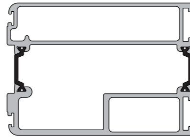
KAS7503 100mm Concealed Vertical Rod Stile
