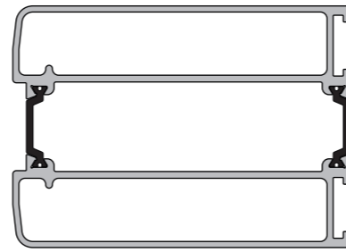
KAS7502 100mm Slave Stile
