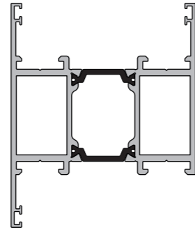
KAS762 Top Rail
