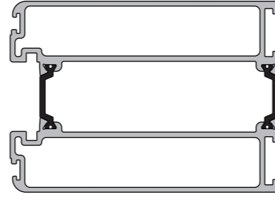
KAS7501 100mm Lock Stile
