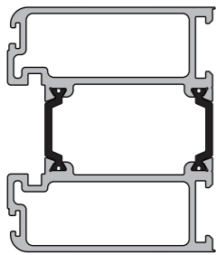
KAS764 Mid Rail
