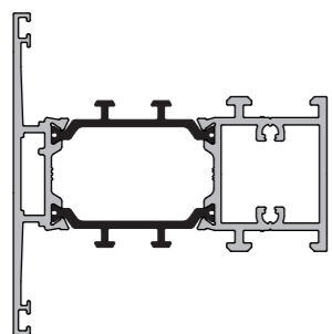
KAS6106 Wide Mullion / Transom
