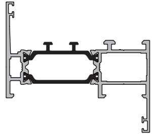
KAS6102 Odd Leg Outer Frame (Bead Out)
