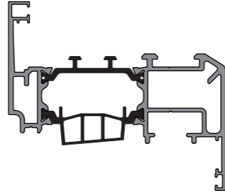
KAS6108 Tilt Before Turn Vent
