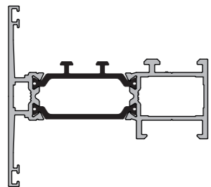
KAS6104 Odd Leg Outer Frame (Bead In)
