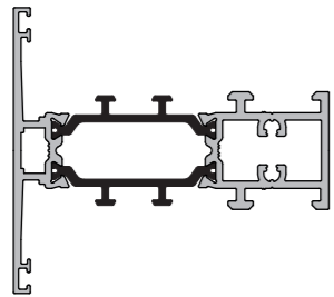
KAS621 Cill Base
