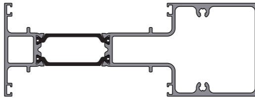
KAS6113 Expansion Coupler
