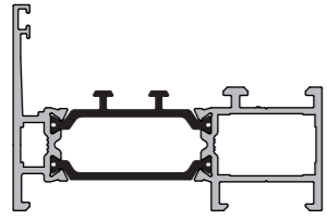
KAS6107 Casement Vent Adapter
