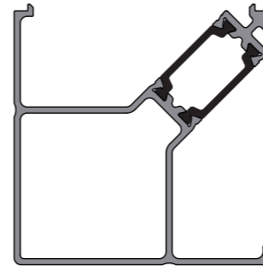
KAS6112 75mm Corner Post
