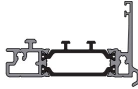
KAS6107 Casement Vent Adapter
