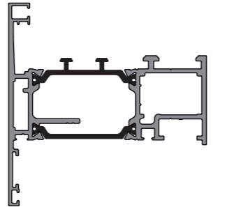
KAS6113 Expansion Coupler
